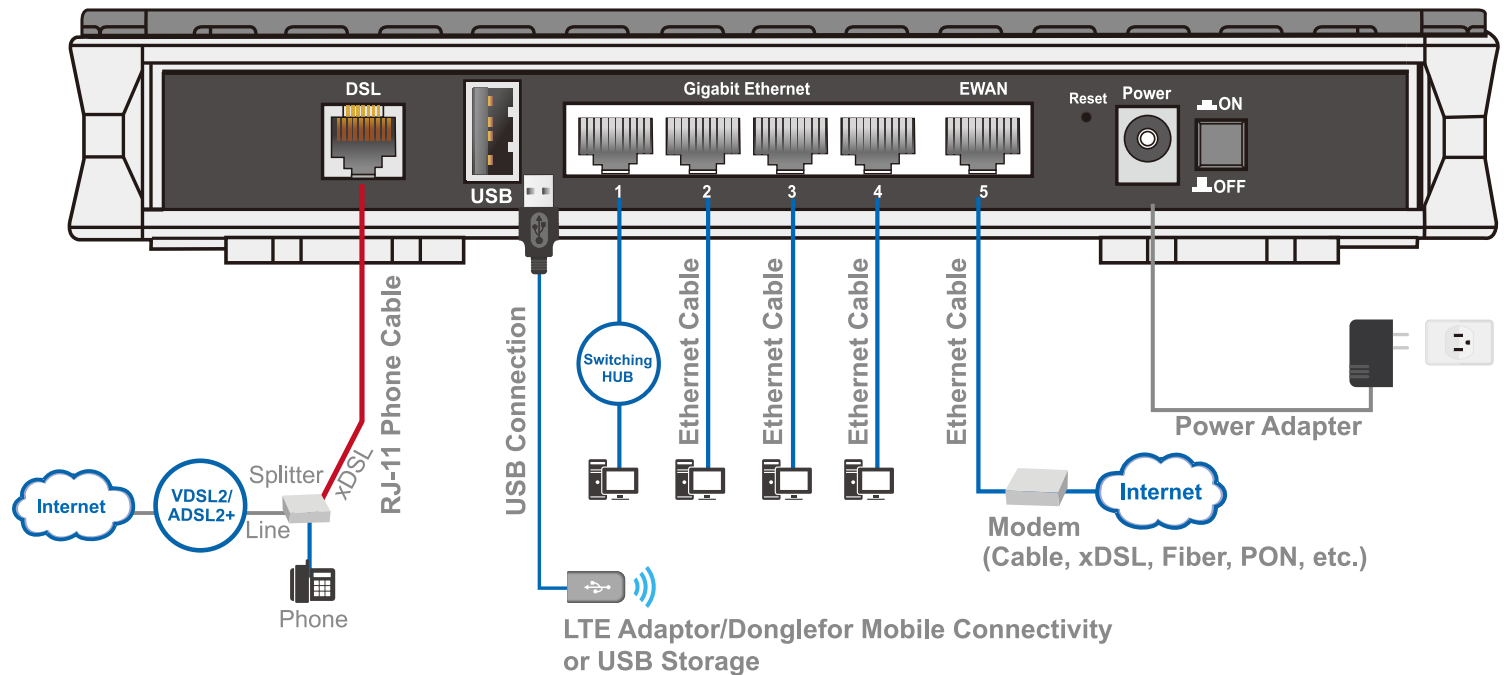
BiPAC 8900X R3 LTE VDSL2/ADSL2+ VPN Firewall Router
